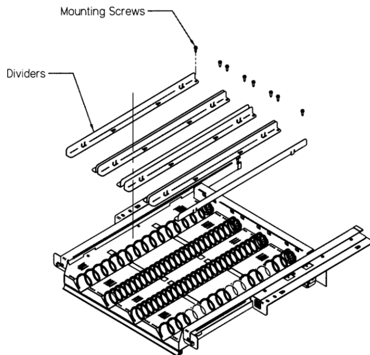
Figure 5.4 1.5" HELIX TRAY
